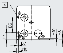
View B ∅ 18
