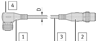
Fig. 3 NEBU-M12W5...-M12G...
