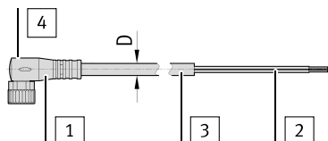
Fig. 4 NEBU-M8W4L...-LE2
