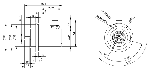
Connector outlet radial
