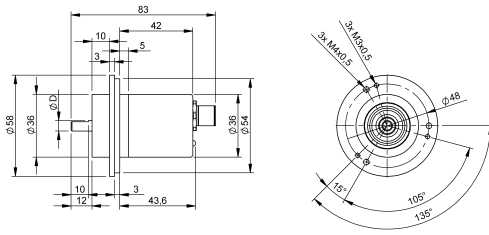
Connector outlet axial
