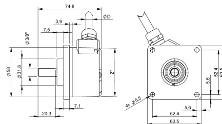
Cable outlet radial
