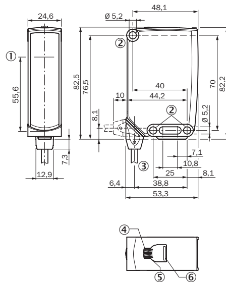
Figure 11: Dimensional drawing 1, cable
