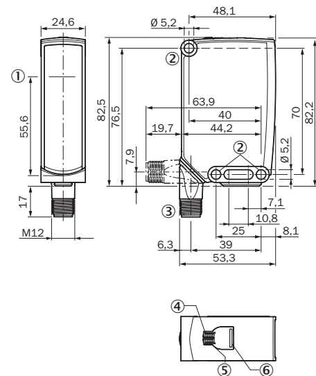
Figure 12: Dimensional drawing 2, male connector
