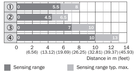
Figure 8: Bar graph 3: Fine triple reflectors
