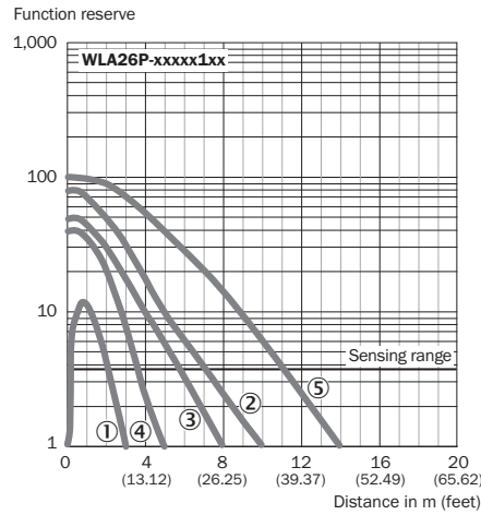
Figure 9: Characteristic line 4: Chemical-resistant reflector
