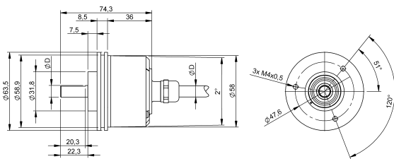
Cable outlet axial
