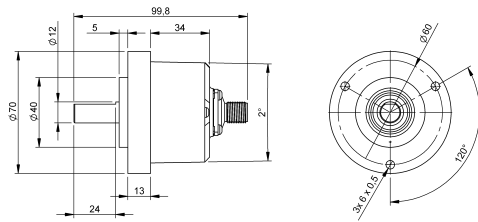
Connector outlet axial
