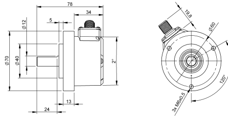
Connector outlet radial
