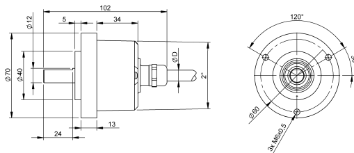
Cable outlet axial
